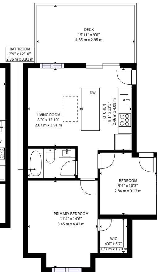
UPPER UNIT
