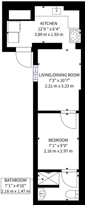
BASEMENT
