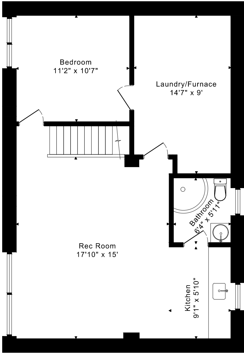
LOWER FLOOR 810 SQUARE FEET
