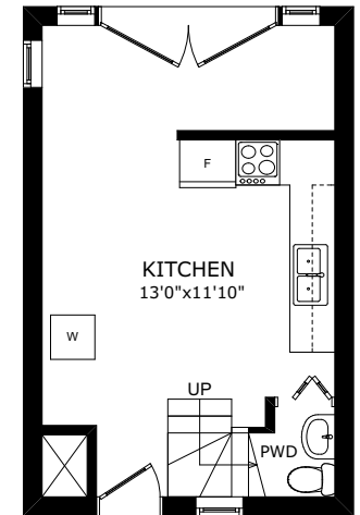
UPPER LEVEL (COACH HOUSE) CLG: 8'0"
