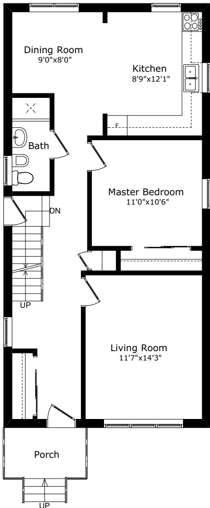
MAIN FLOOR
