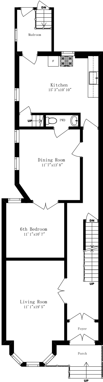
MAIN FLOOR
