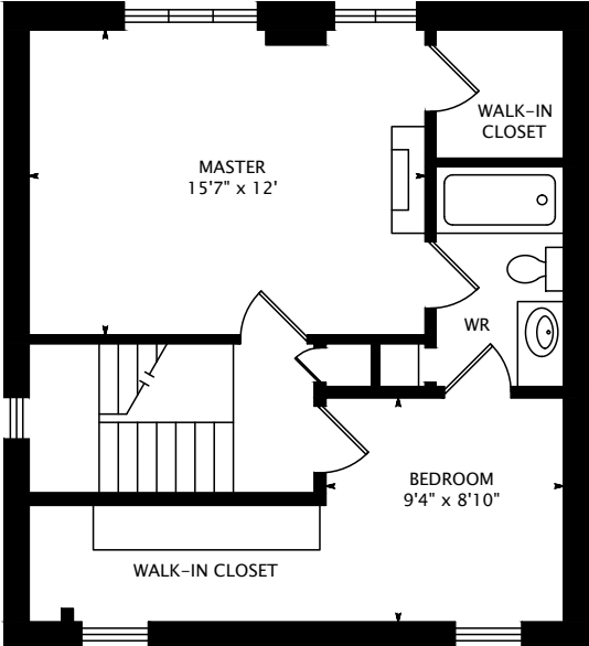
SECOND FLOOR 584 SQUARE FEET
