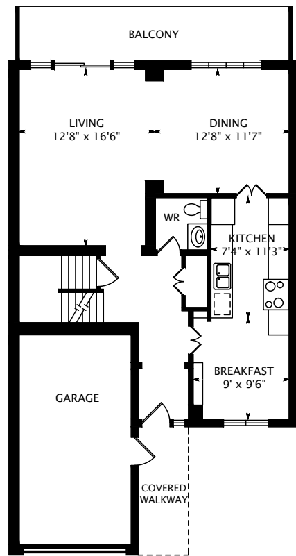
MAIN FLOOR 839 SQUARE FEET
